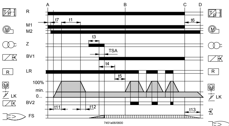
2-stage expanding flame burner
